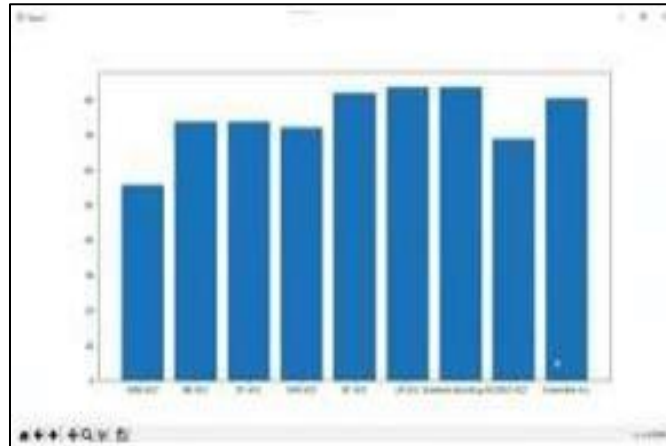
Fig8: Accuracy graph
