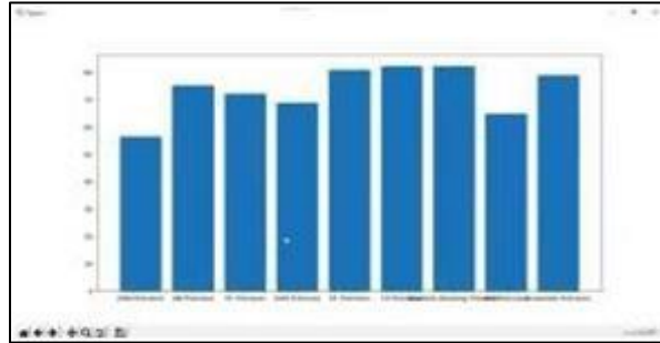
Fig5: Precision graph
