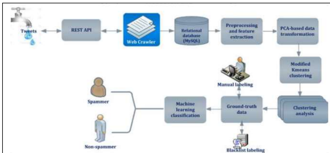
Fig 1: Comment Spam Detection
