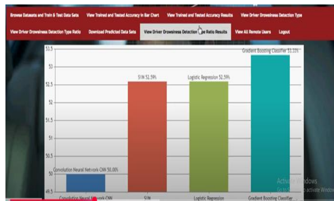
Figure 5 Graph Analysis
