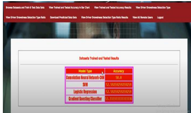
Figure 4 Data Set
