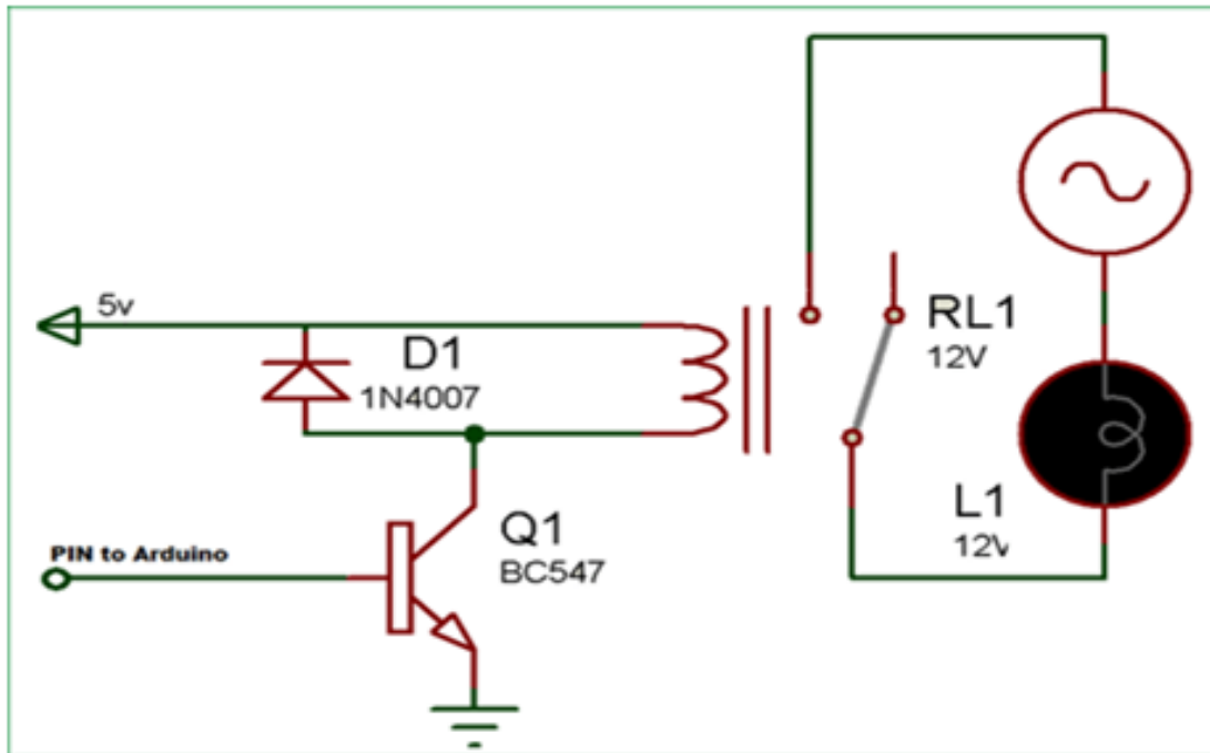
Fig 2: Relay
